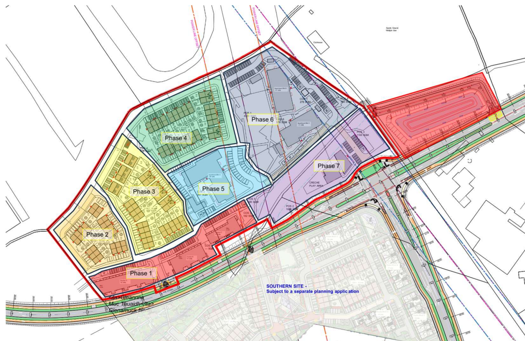
Figure 2-1 Draft Construction Phasing Plan
